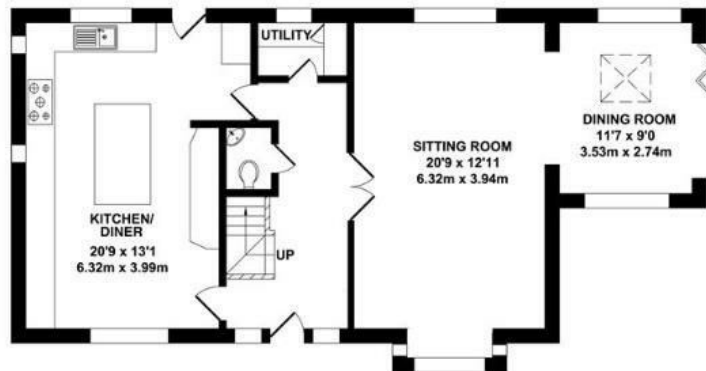
GROUND FLOOR APPROX. FLOOR AREA 856 SQ.FT. (79.52 SQ.M.)
